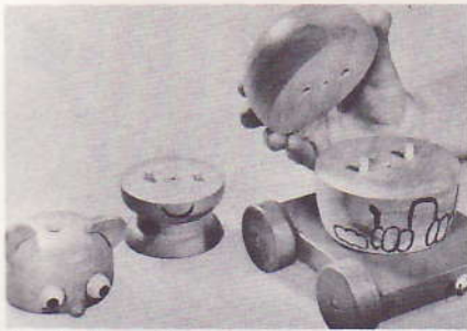
A pair of pegs in each section makes the parts self-aligning when they are stacked in the proper order
