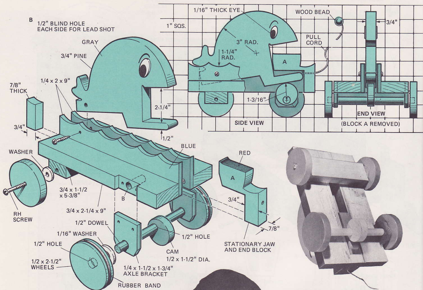
Underside view shows how cam on dowel axle opens, and closes the whale's mouth
